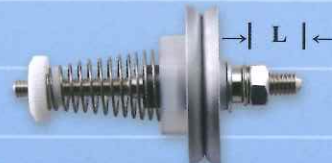
KC1310A (L:14mm)
