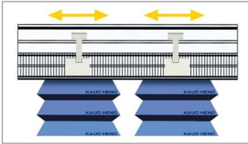
1+1 system knitting operation
